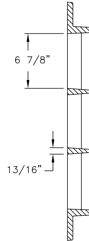
GRATE SECTION
