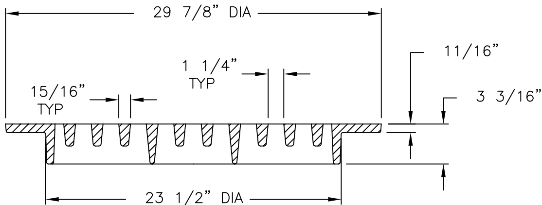
GRATE SECTION
